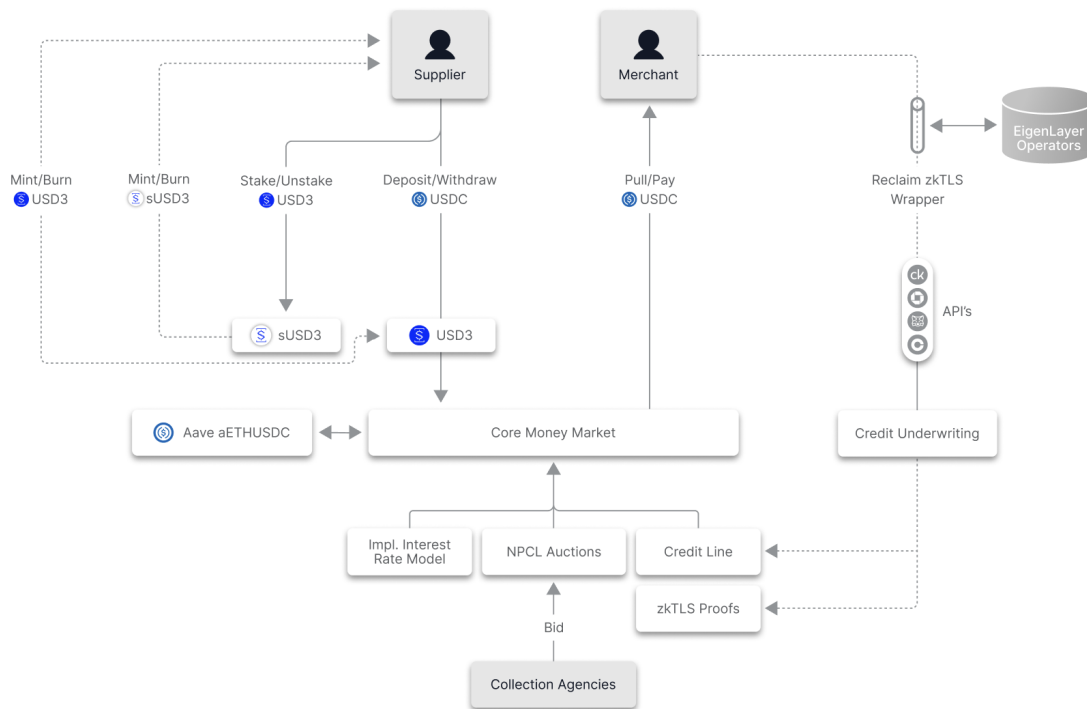
Figure 2: Protocol Architecture
