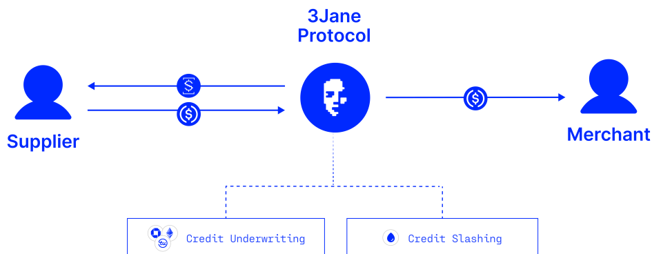
Figure 1: 3Jane Protocol
